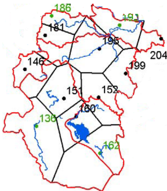
Figure 8: The Ljubljana river basin with precipitation stations and Thiessen polygons
