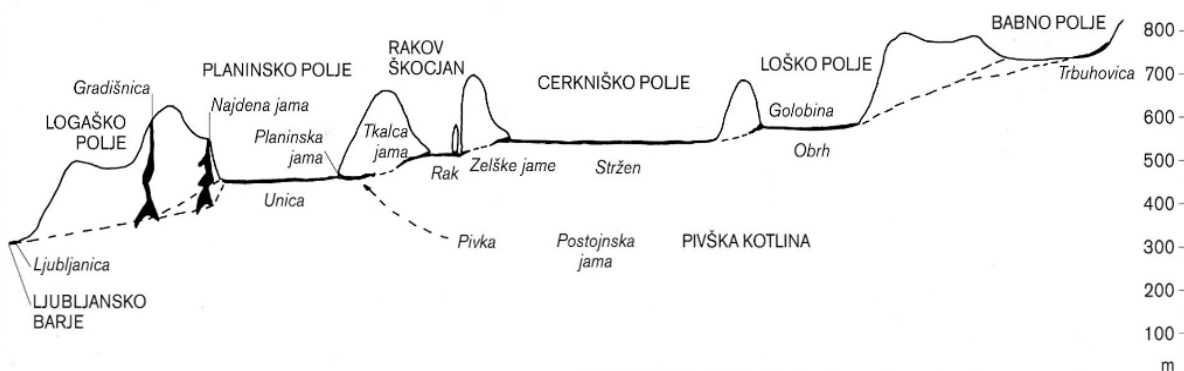
Figure 2: Cross section of river Ljubljana system from Prezid to Vrhnika
